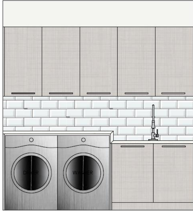
Typical Laundry Elevations
