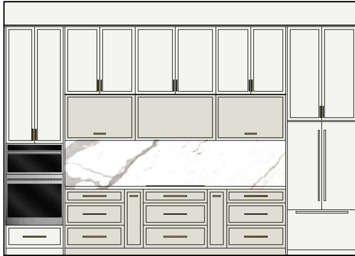
Typical Kitchen & Family Room Elevation Refer to millwork package for all model suite drawings
