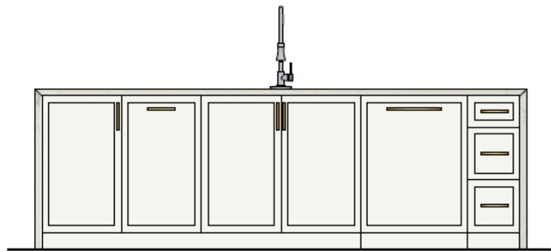
Typical Kitchen Island Elevation
