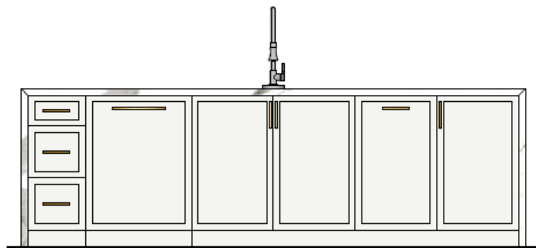
Typical Kitchen Island Elevation Refer to millwork package for all model suite drawings
