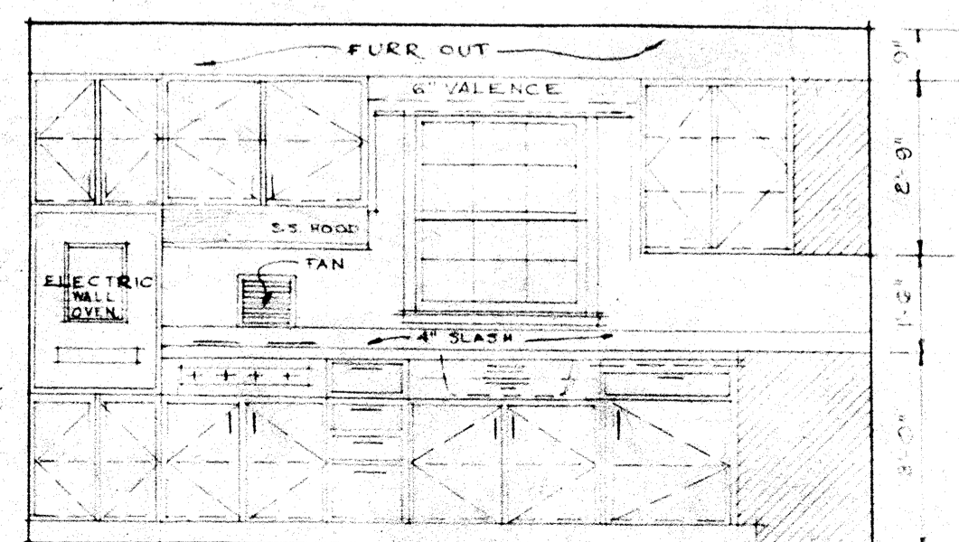
OPTIONAL D.W. LOCATION ELEVATION "A" 3/8" = 1"
