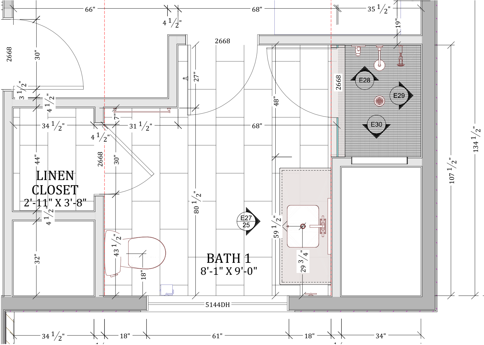
PLAN VIEW SHOWN AT 1/2" = 1"
