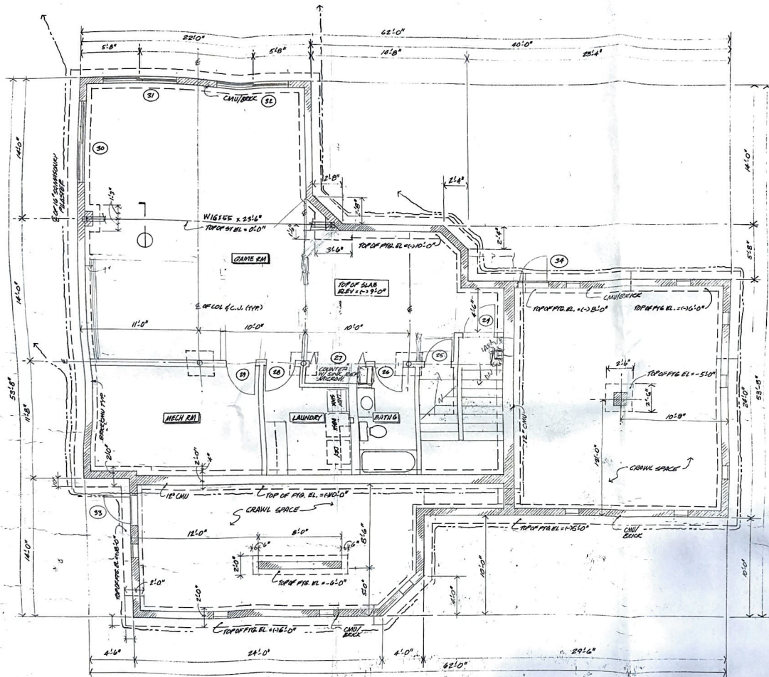
BASEMENT/FLR - FOUNDATION PLAN SCALE: 1/8" = 1'-0"
