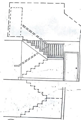
6 STAIR WLEV. SCALE 1/4"=1'-0"
