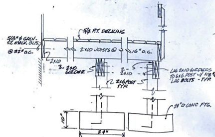
5 TYP. DECK DTLS. SCALE: 3/4" = 1'-0"
