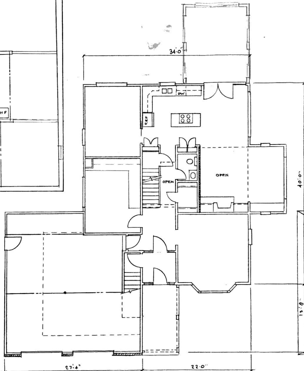
FIRST FLOOR PLAN 1/8"=1'-0"
