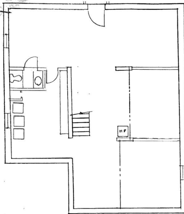
BASEMENT PLAN 1/8"=1'-0"
