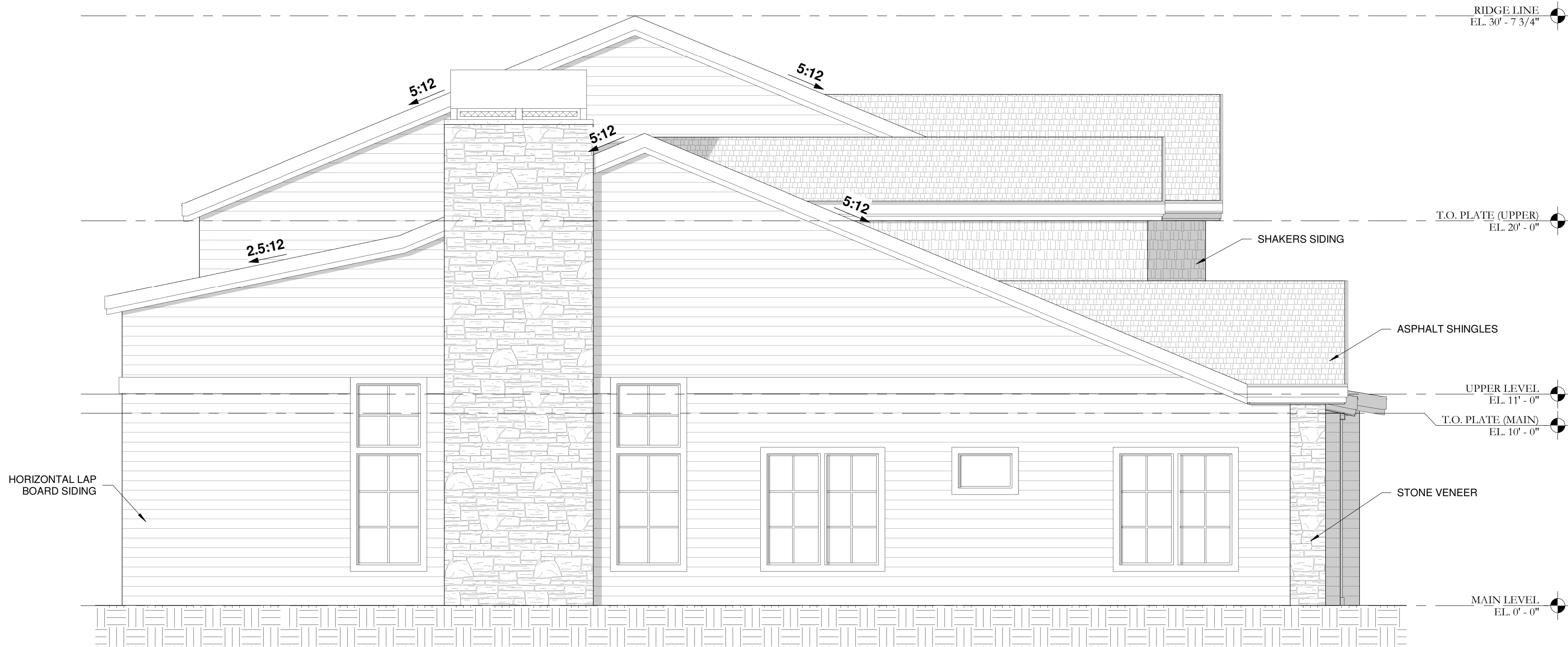
1 LEFT SIDE ELEVATION SCALE: 1/4" = 1'-0"
