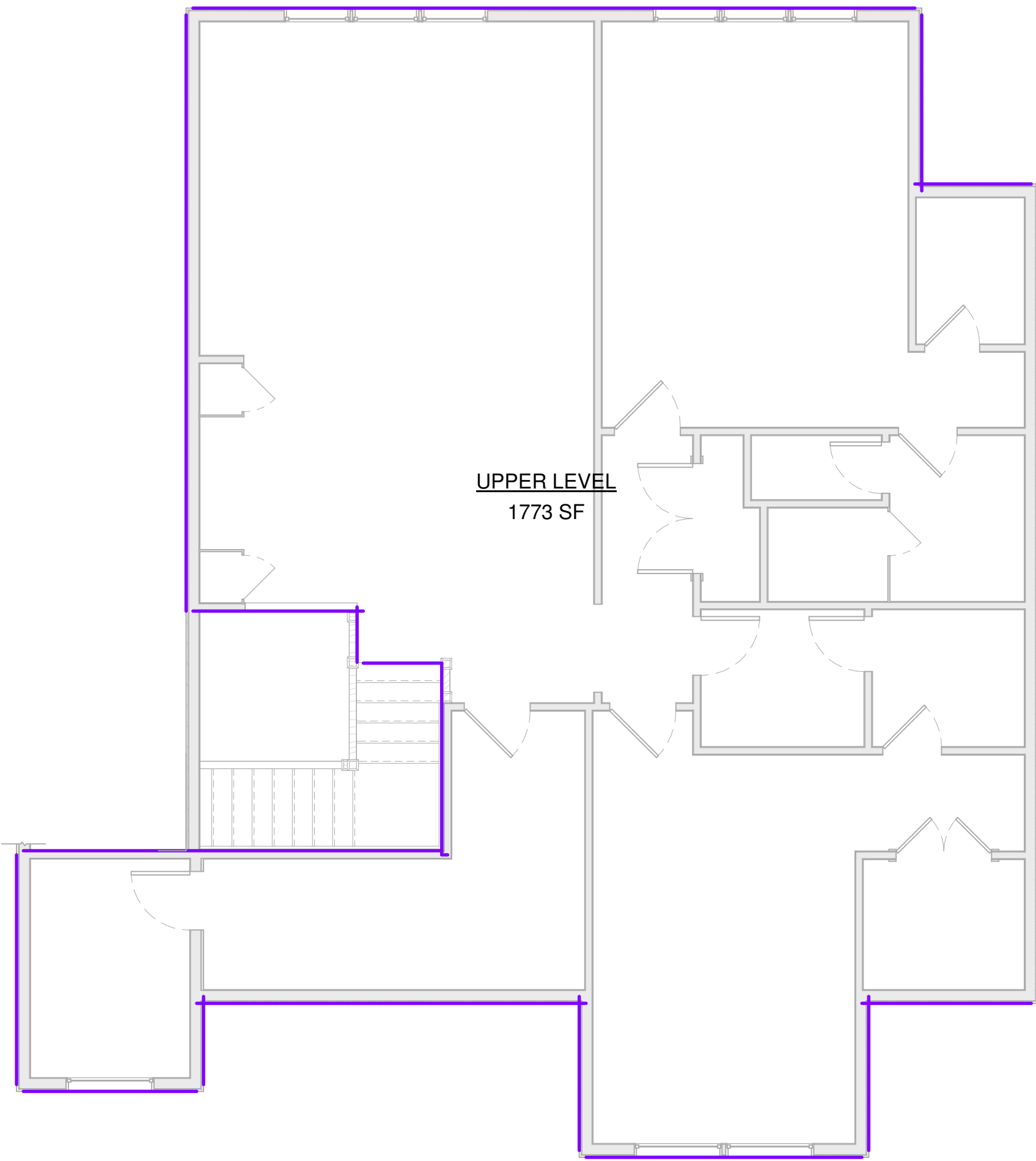
2 UPPER LEVEL AREA PLAN SCALE: 3/16" = 1'-0"
