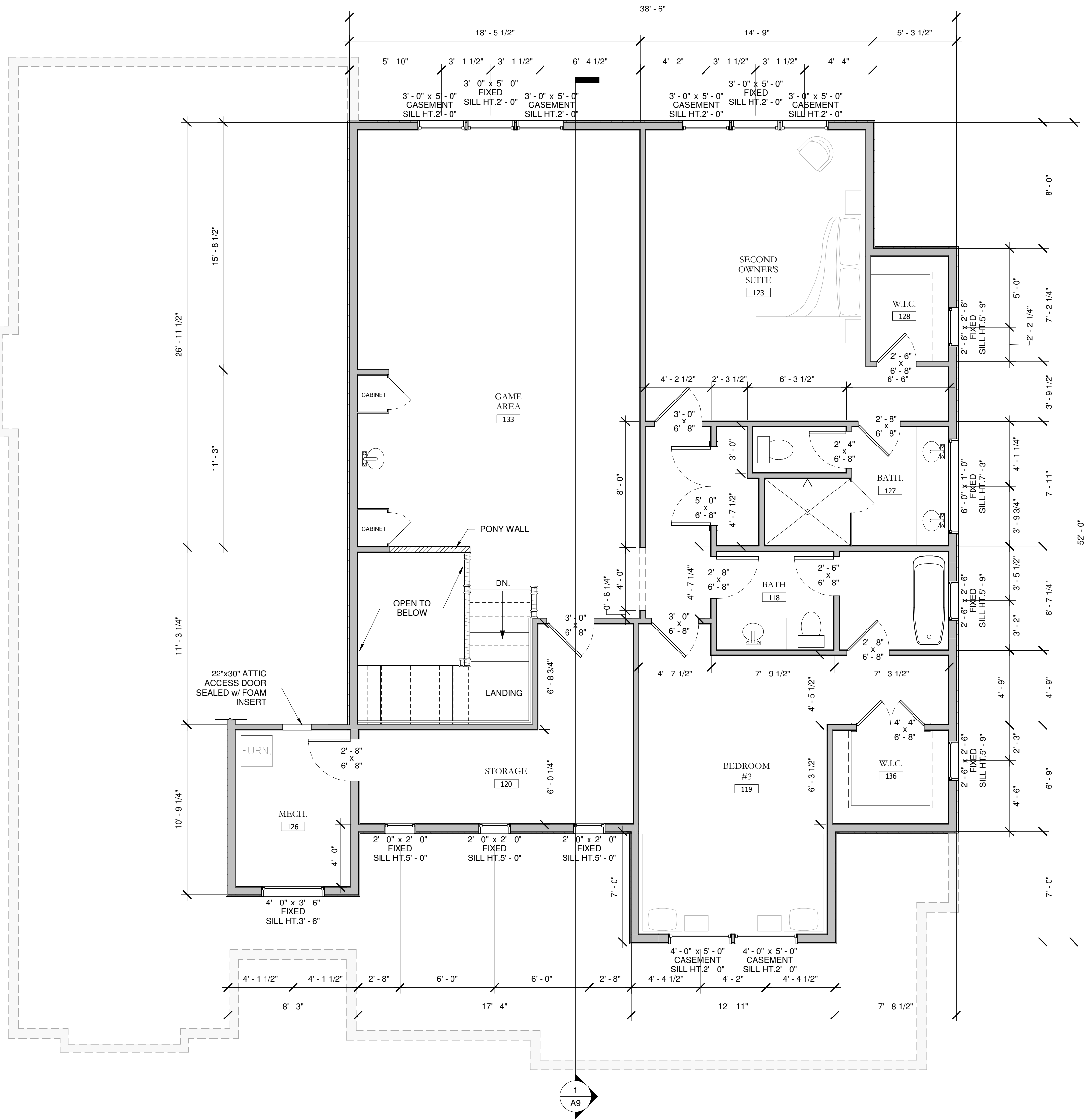
1 FLOOR PLAN - UPPER LEVEL SCALE: 1/4" = 1'-0"
