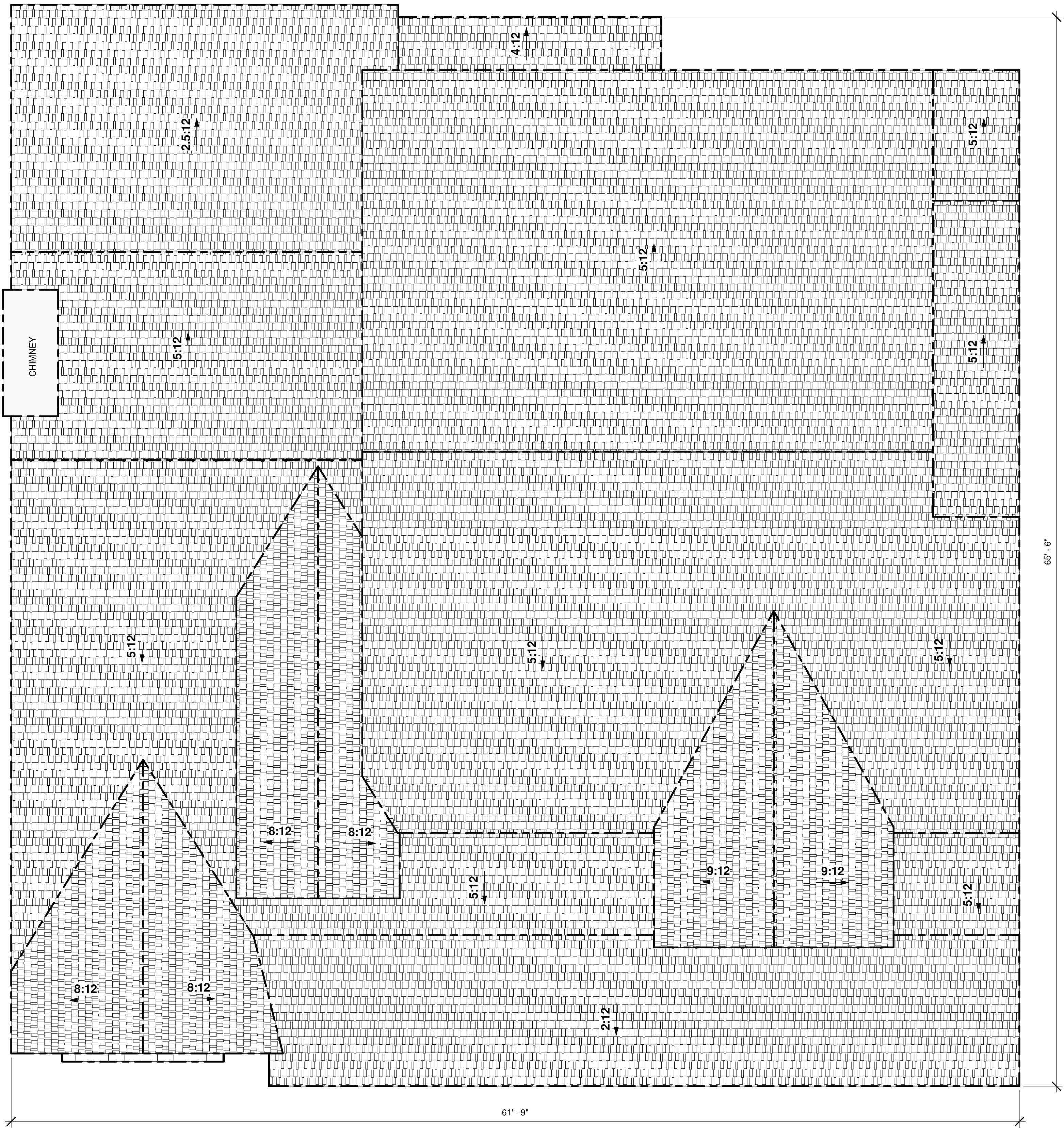
1 ROOF PLAN SCALE: 1/4" = 1'-0"
