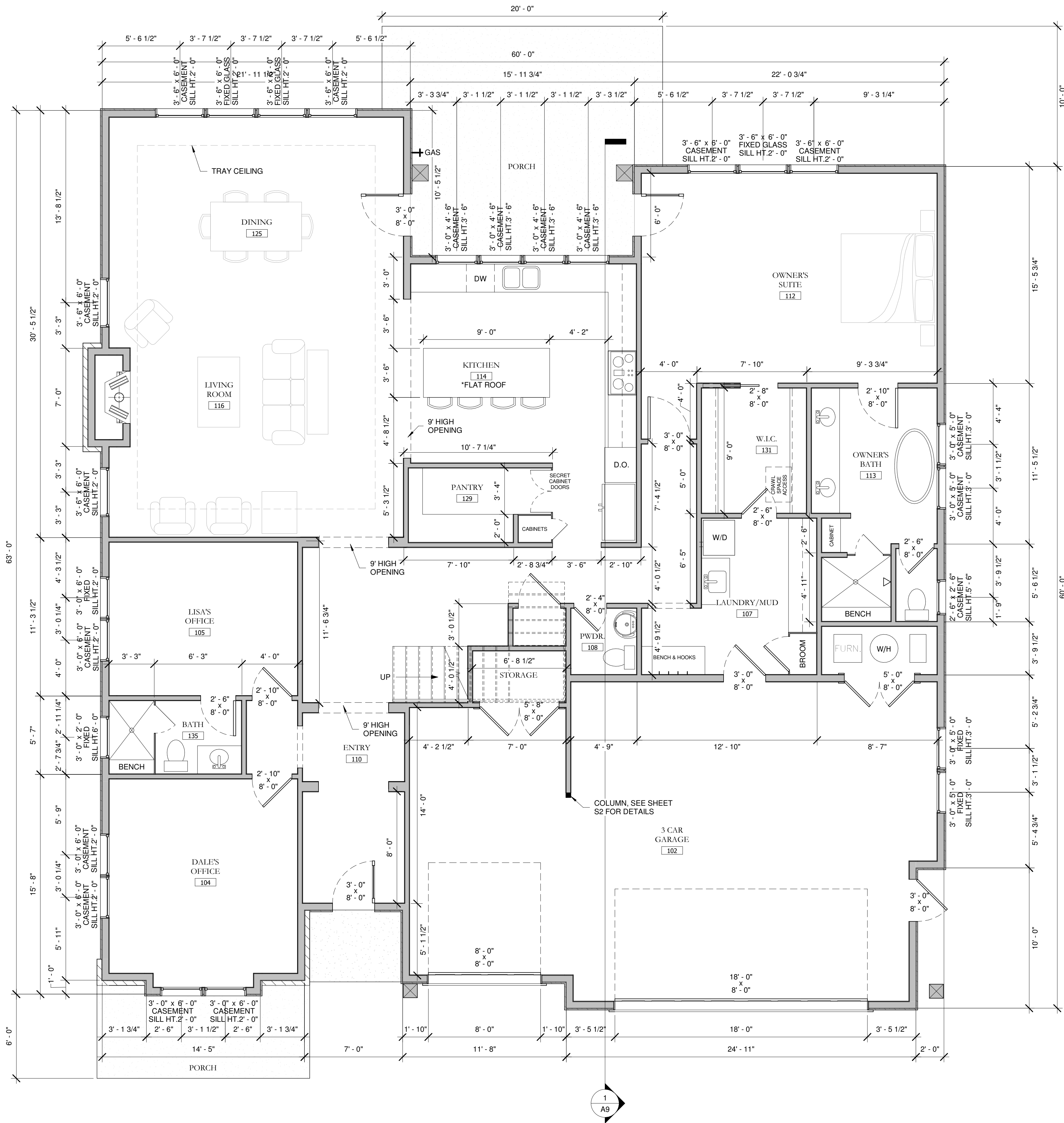
1 FLOOR PLAN - MAIN LEVEL SCALE: 1/4" = 1'-0"
