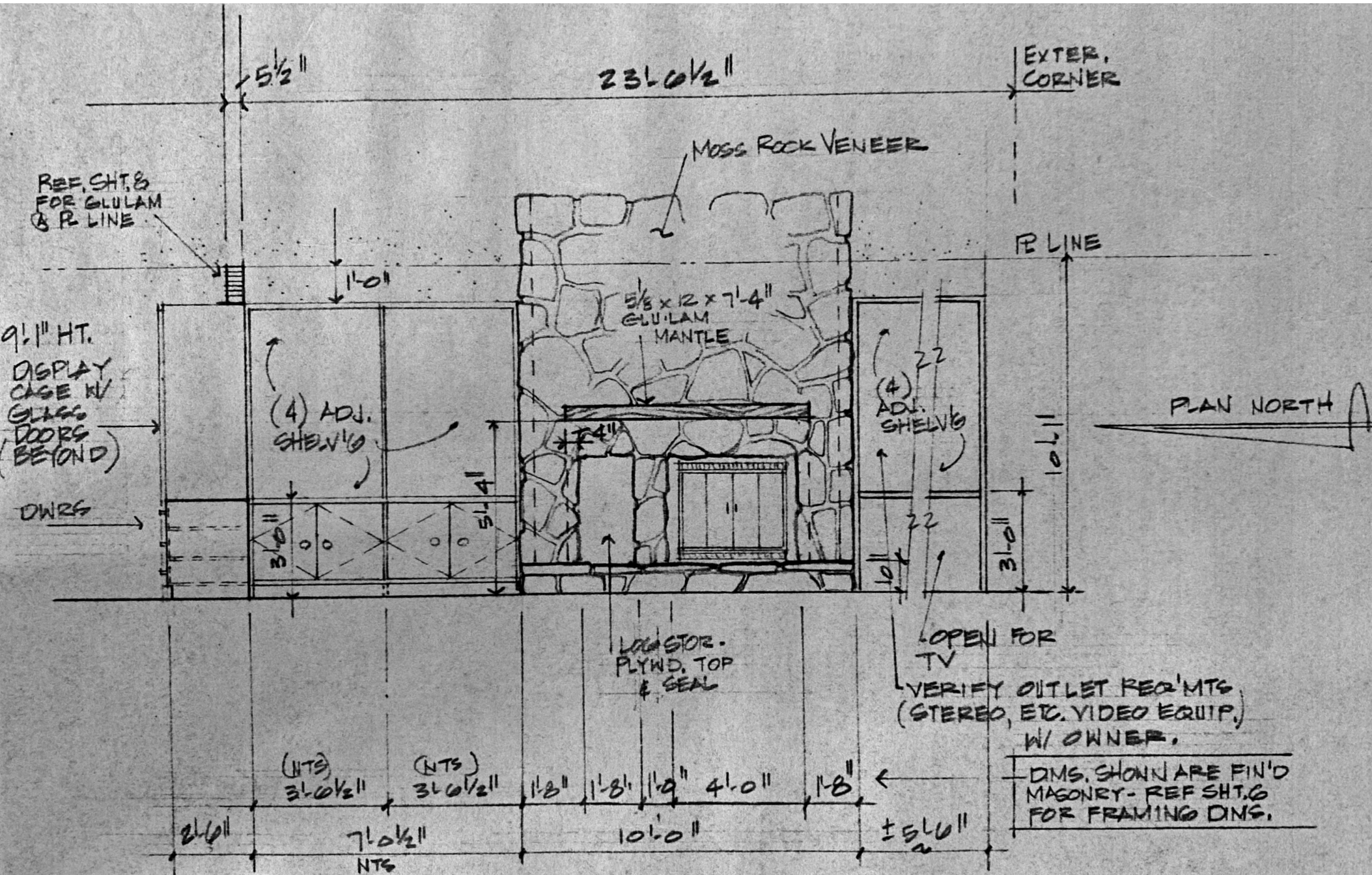
A. ELEVATION. SOUTH WALL. LIVING AREA. MAIN LEVEL 1/4" = 1'-0"
