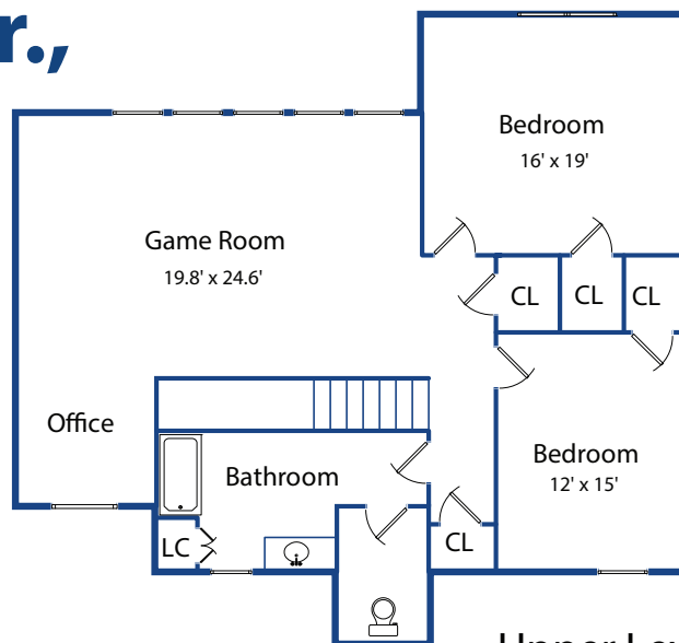
Upper Level
