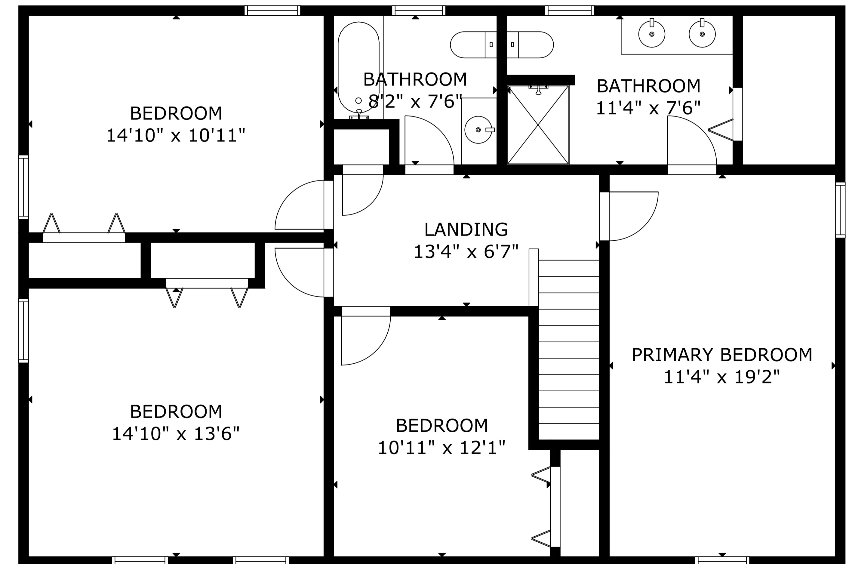
SECOND FLOOR
