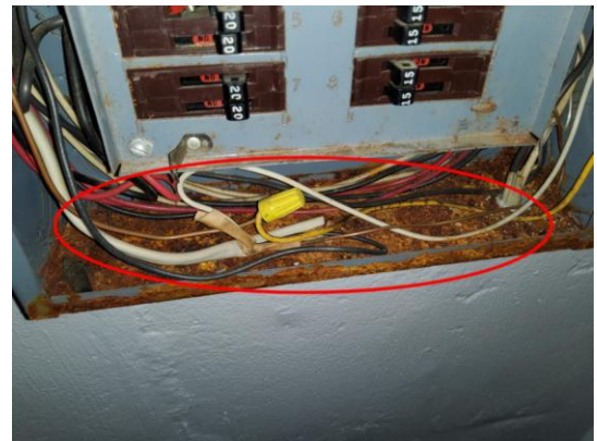
Photo 15: Rusted Panel.
