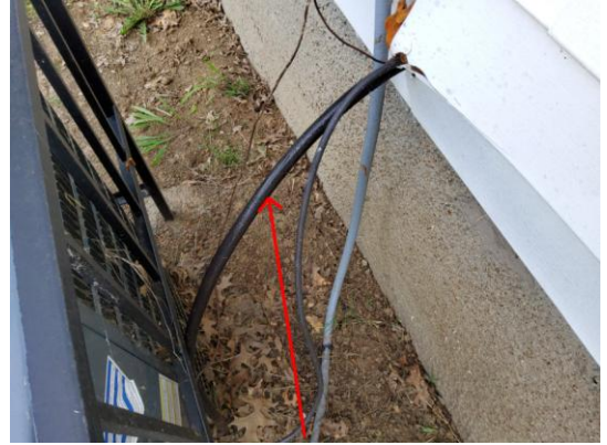
Photo 21: Insulation Missing on Refrigerant Lines .
