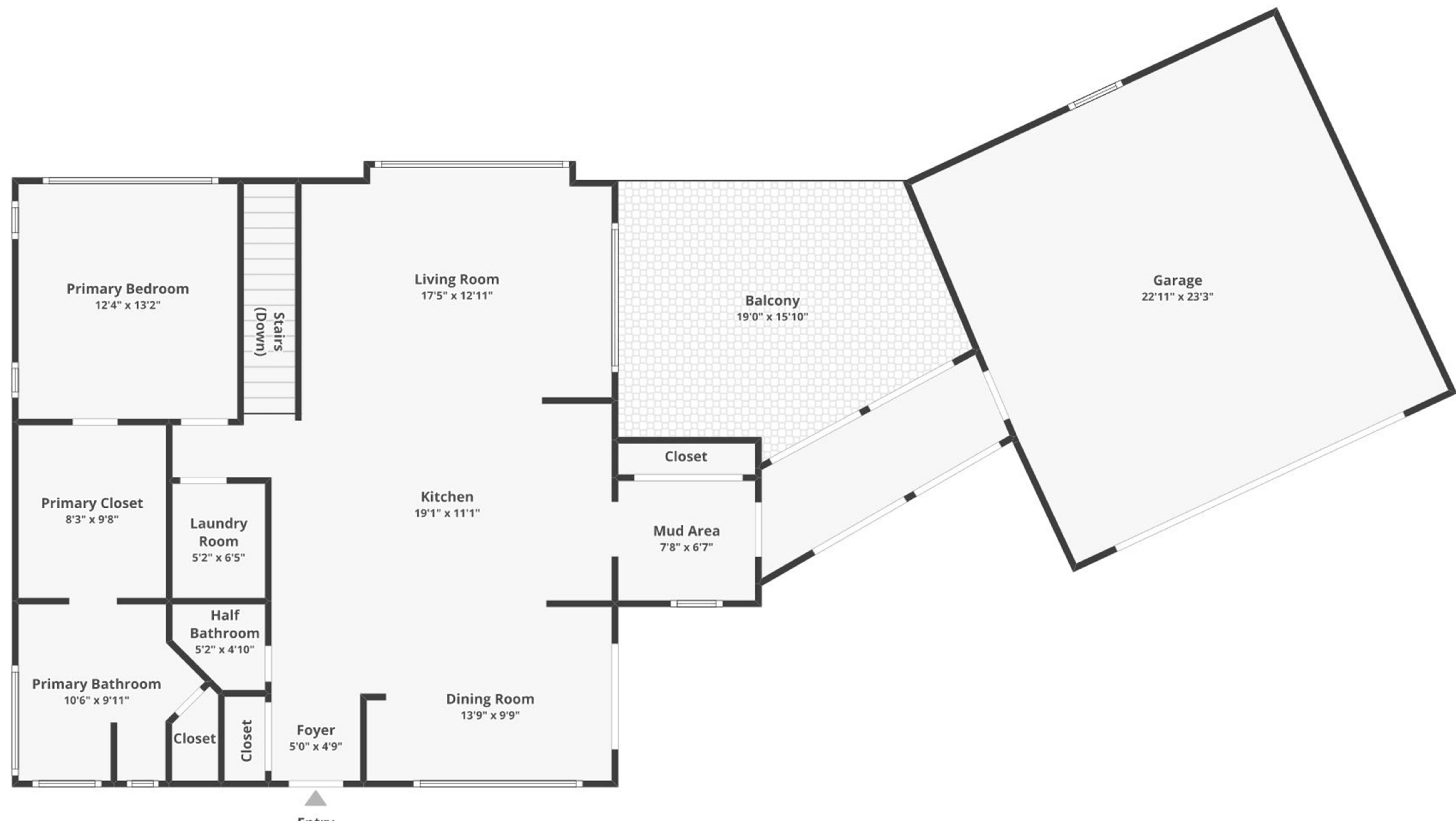
Main Level
