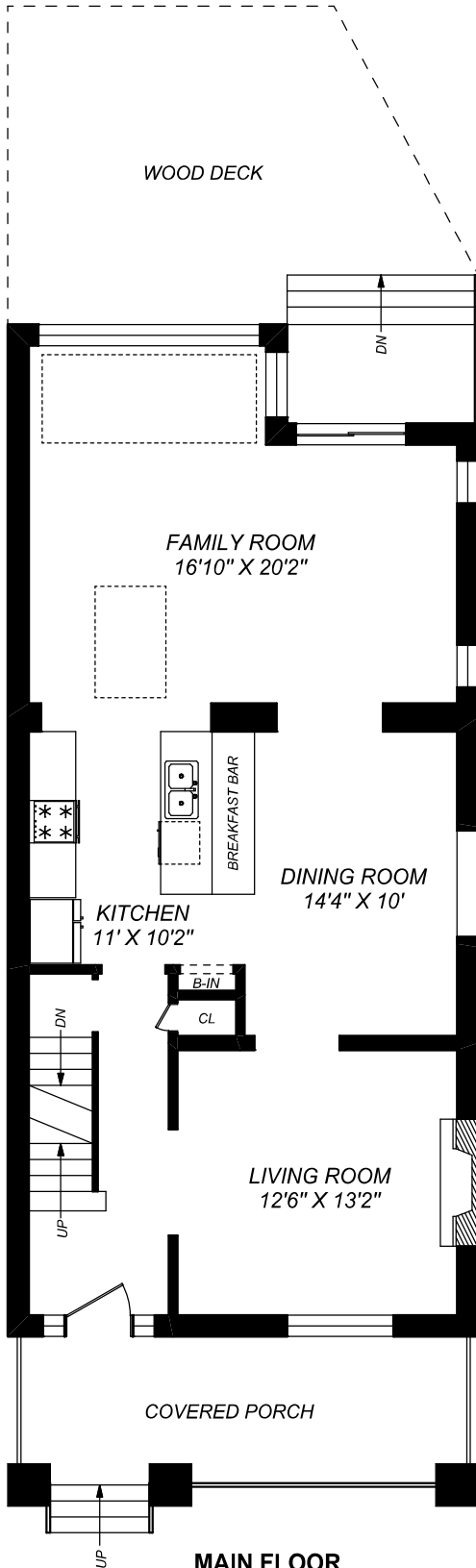
MAIN FLOOR 1008 SQUARE FEET (CEILING HEIGHT : 8'-3")
