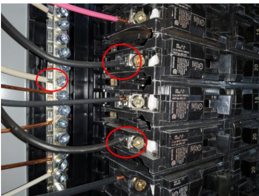
Photo 18: Aluminum Wiring.
